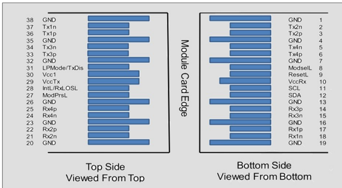
Pin Diagram
