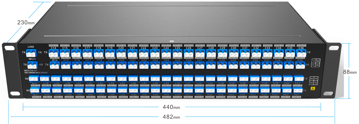
96CH DWDM 1U RACK
