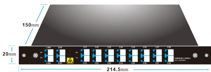
LGX BOX Plug in 4-Slot 1U Rack
