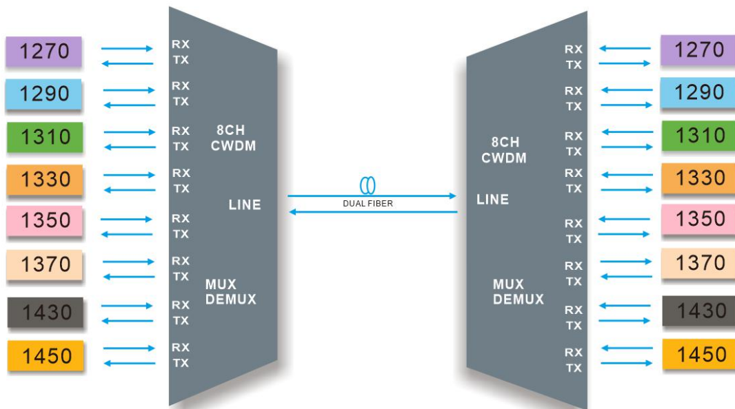
8CH CWDM MUX DEMUX Dual fiber transmission
